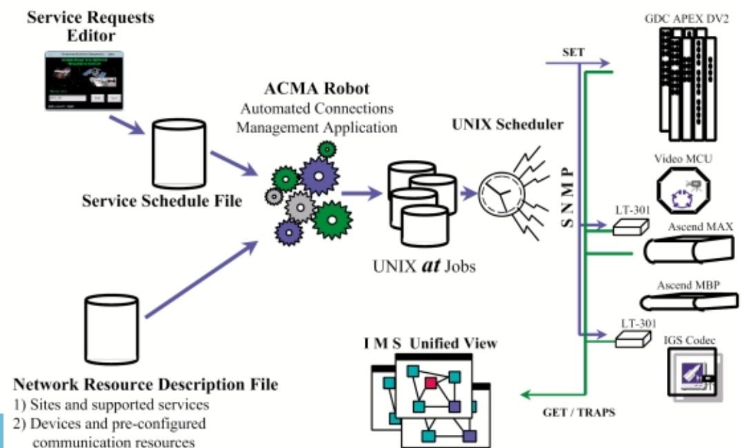
Figure 8. An Automated Connections Management Application (ACMA)
